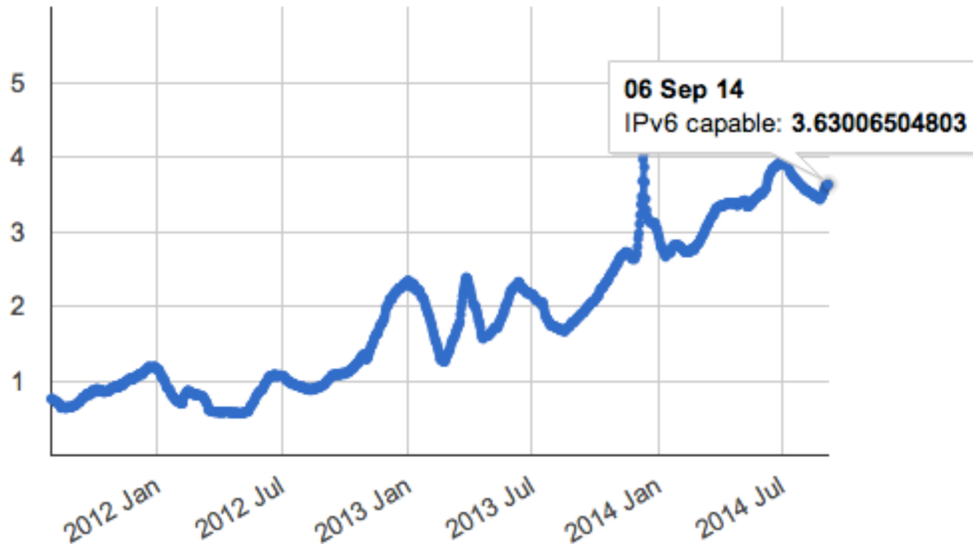
IPv6 Preference by Month
