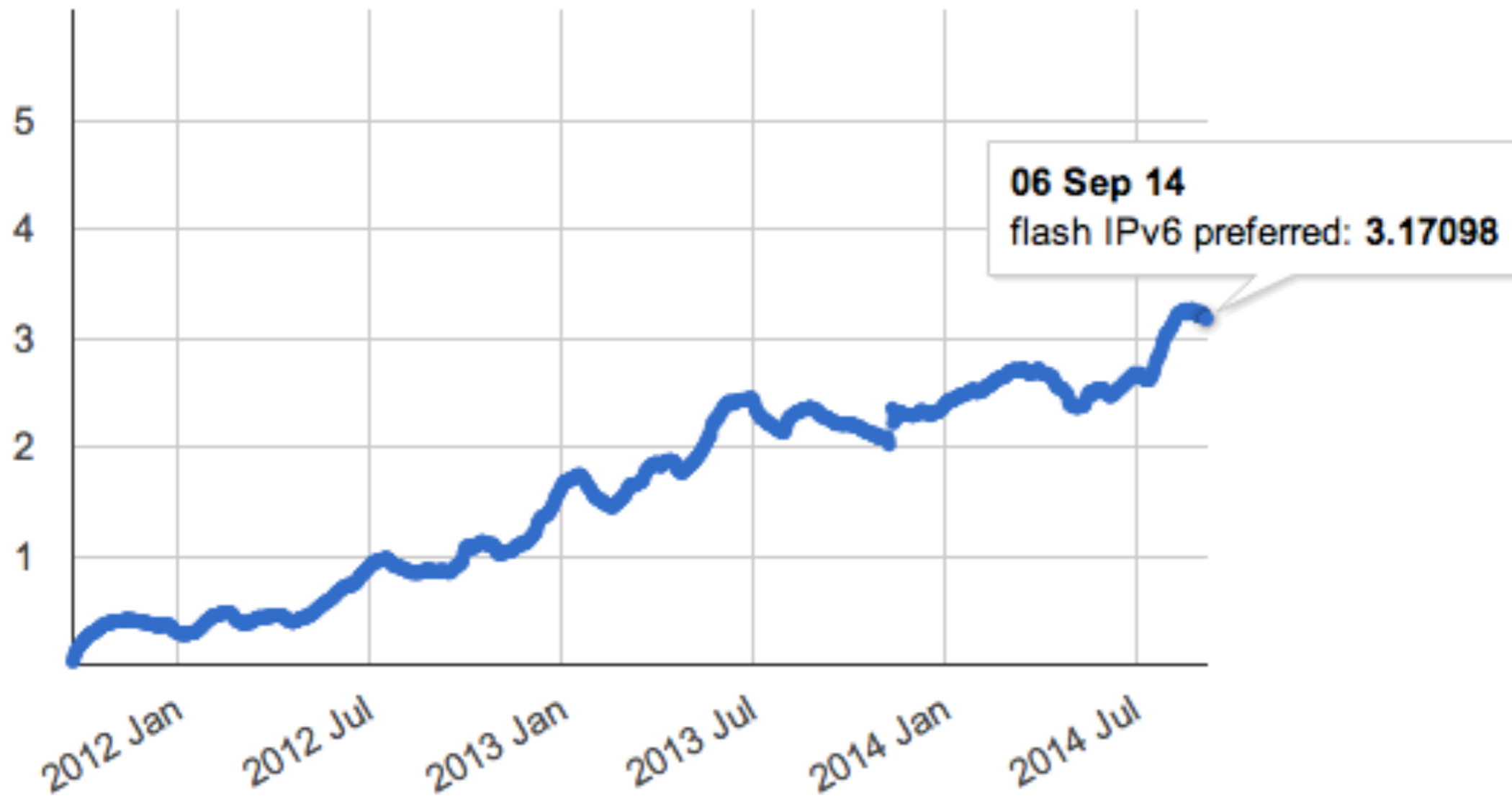
IPv6 Preference by Month
