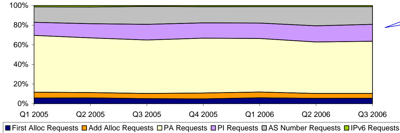
Distribution of % of Resource Request Types
