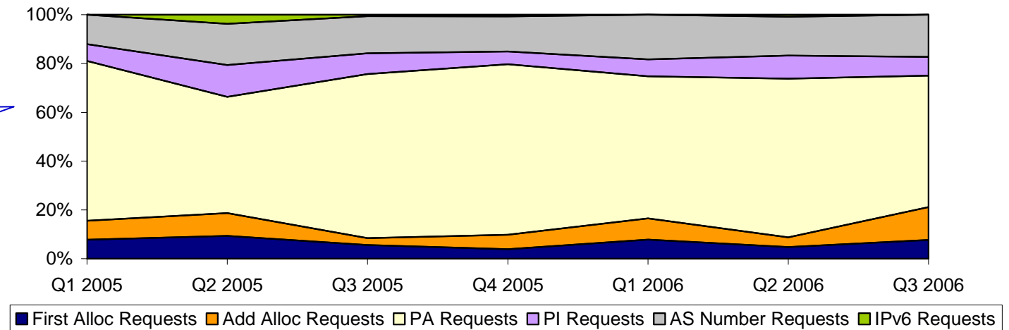
Distribution of % of Resource Request Types
